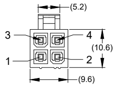
4-PIN FEMALE MATING FACE
